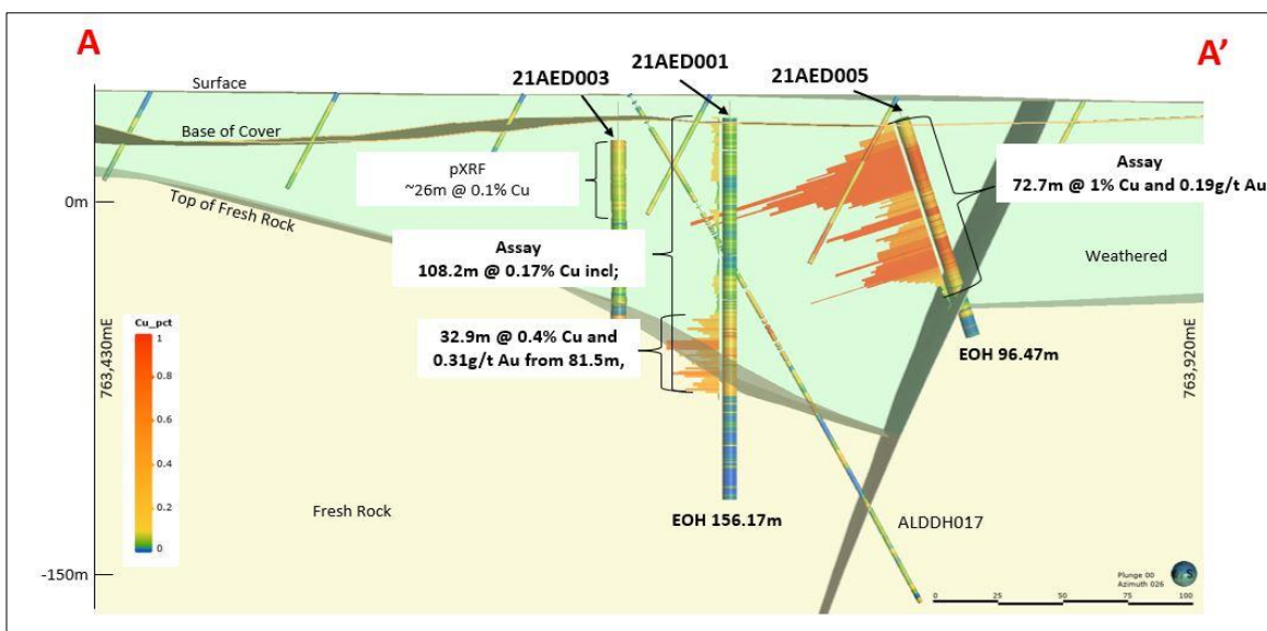
Figure 8: Cross section showing 21AED001, 21AED003 and 21AED005
